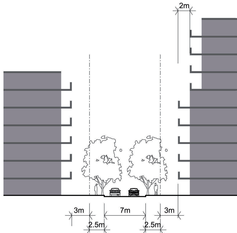
Street section
