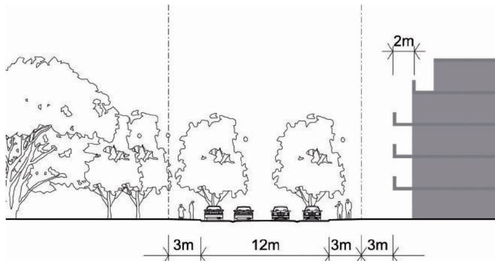
Street Section
